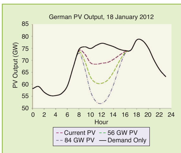
figure 3. The demand and net demand in Germany with various levels of installed PV capacity.
