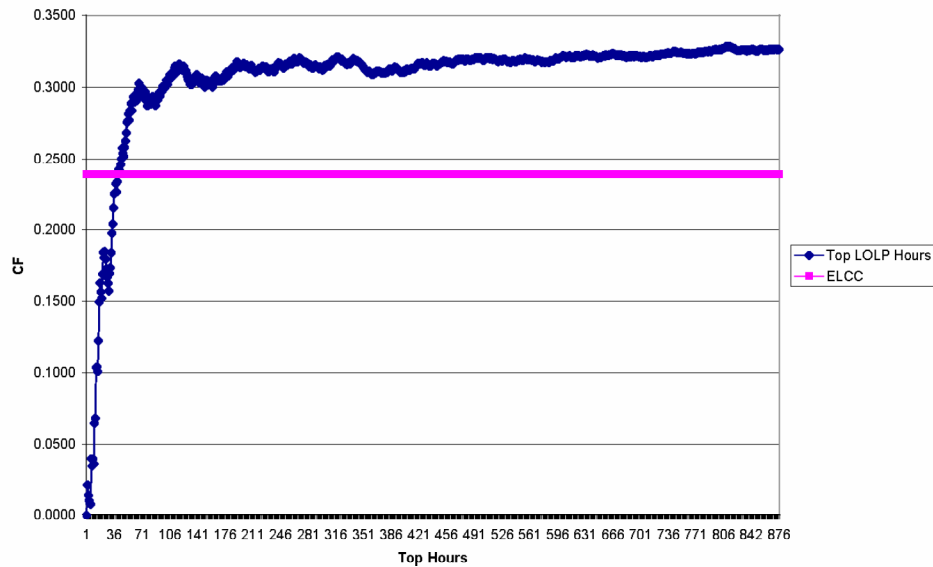
Figure 3.16 Wind capacity factor in San Geronio region.
