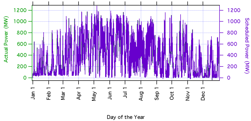
Figure 5.10 Actual and Scheduled Total Wind Generation for the Year
