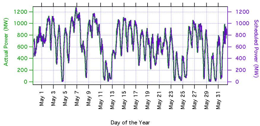
Figure 5.11 Actual and Scheduled Total Wind Generation in May
