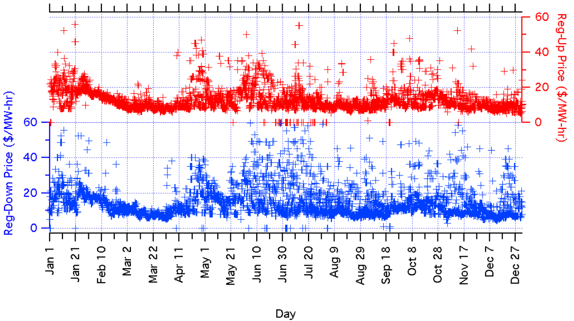
Figure 2.22 CalSO regulation market prices in 2002.
