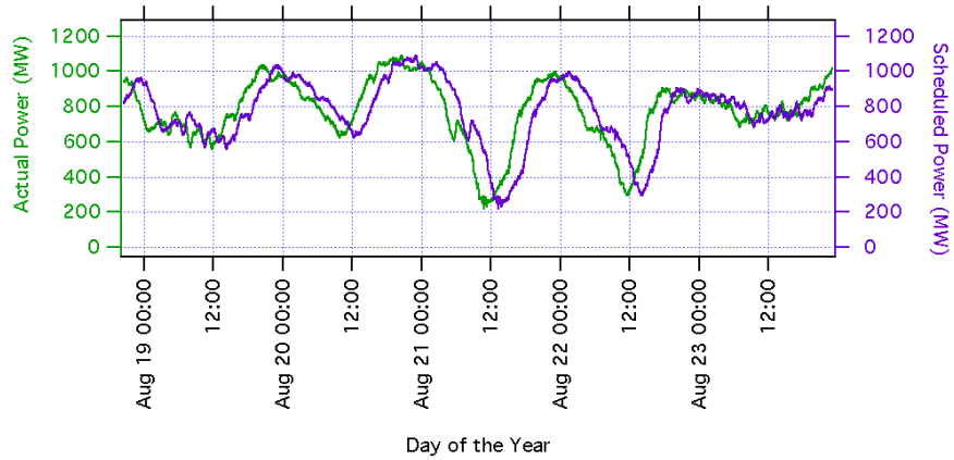
Figure 5.12 Actual and Scheduled Total Wind Generation for Several Days in August
