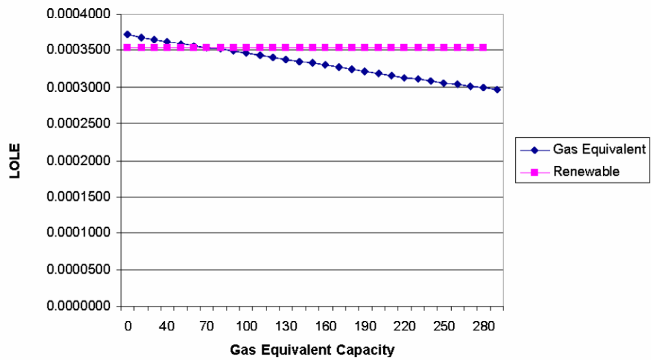
Figure 3.10 Wind reliability curve in San Gorgonio region.
