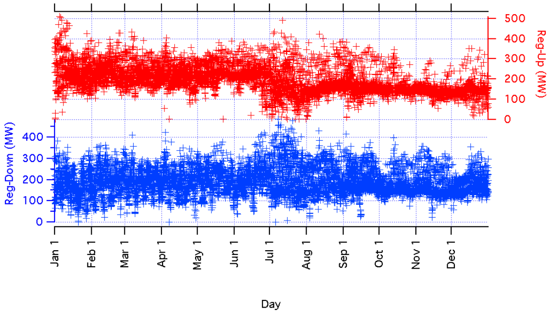
Figure 2.21 CalSO regulation purchases in 2002.
