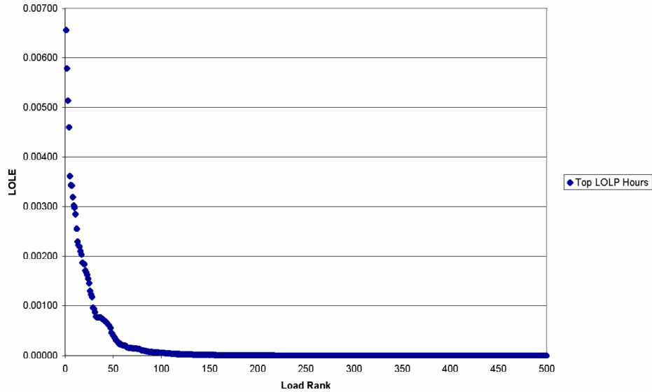
Figure 3.1 Reliability and top 500 hours ranked by load/LOLP.
