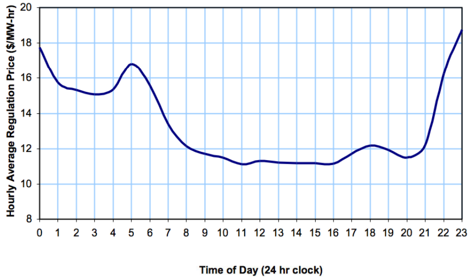
Figure 4.8 Hourly weighted average regulation prices were highest at night when supplying generators incur costs when moving up in order to create room to regulate down.
