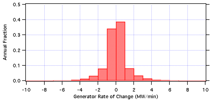
Figure 2.19 Rate of change histogram of power generation of the wind plants in the San Geronimo region for 2002.
