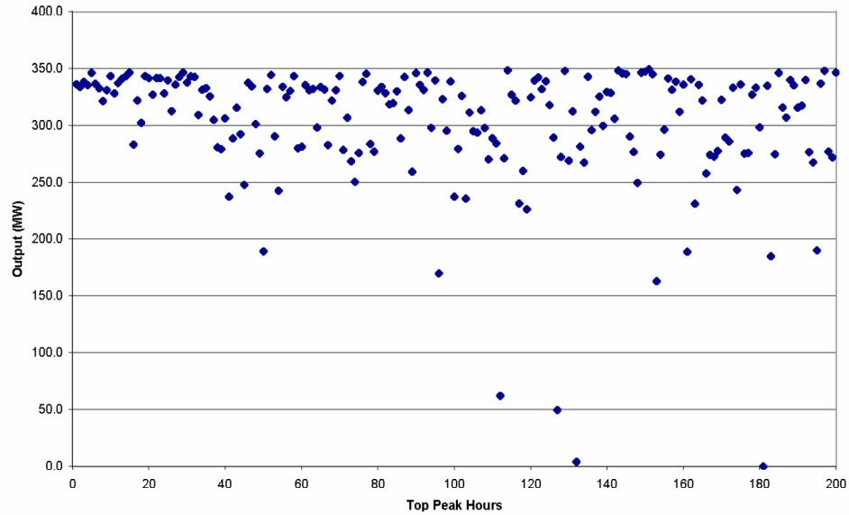
Figure 3.8 Solar output during the top 200 load hours.
